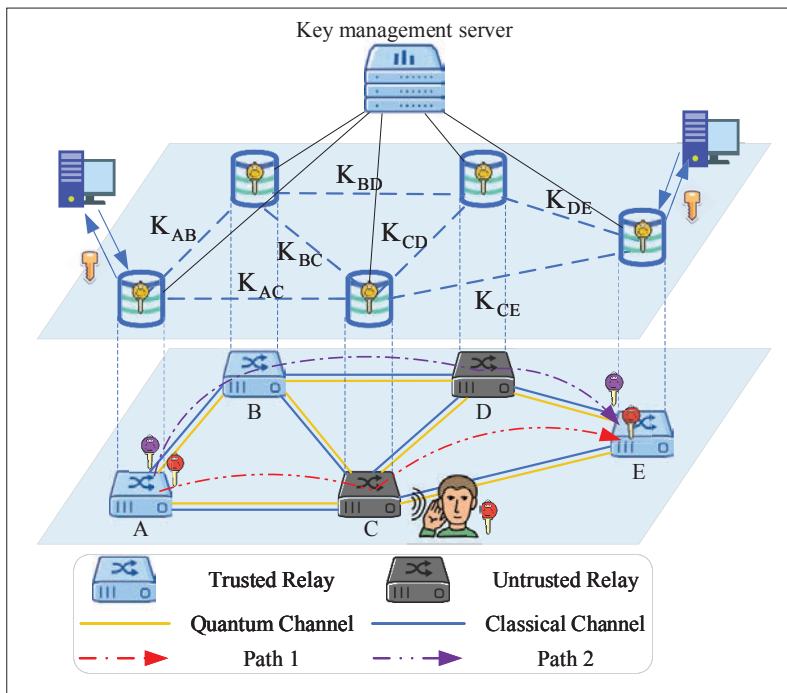
FIGURE 2. A typical structure of a partially-trusted relay QKD network. In order to ensure the security of the global key, two paths are used for key distribution. The final key is reconstructed from the keys distributed by the two paths.
