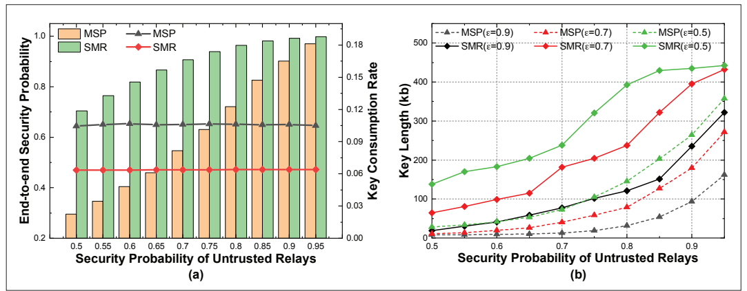
FIGURE 5. The impact of different security probabilities of untrusted relay nodes: a) End-to-end security probability and key consumption rate; b) Length of the global key. The number of trusted relay nodes is set to 10.
