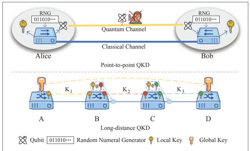
FIGURE 1. The illustration of point-to-point QKD and long-distance QKD.
