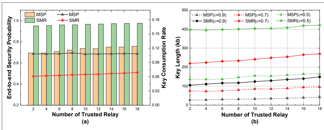
FIGURE 6. The impact of different number of trusted relay nodes: a) End-to-end security probability and key consumption rate; b) Length of the global key. The security probability of untrusted relay nodes is set to 0.8.
