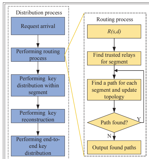
FIGURE 3. The process of end-to-end distribution and segment-based multipath routing algorithm.
